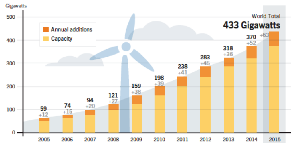
Figure 23. Wind Power Global Capacity and Annual Additions, 2005–2015
