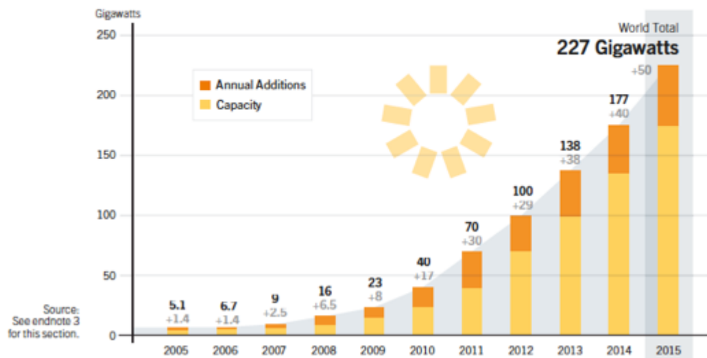
Figure 14. Solar PV Global Capacity and Annual Additions, 2005–2015
